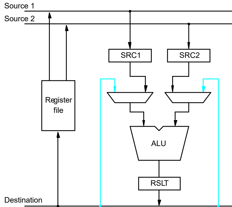
(a) Datapath
